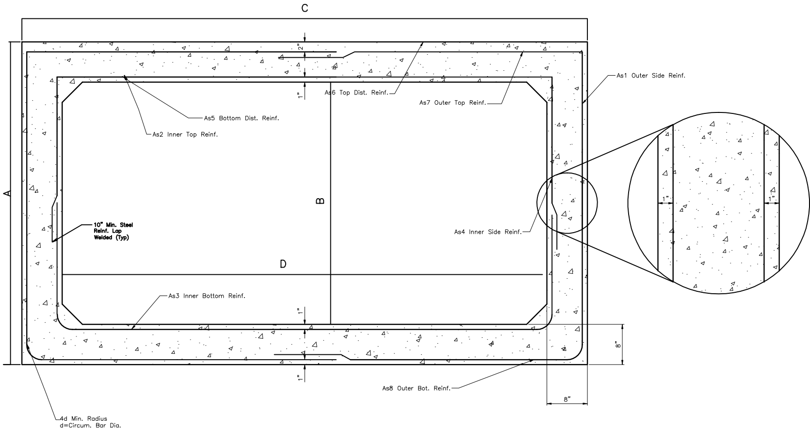
BOX CULVERT TYPICAL SECTION
