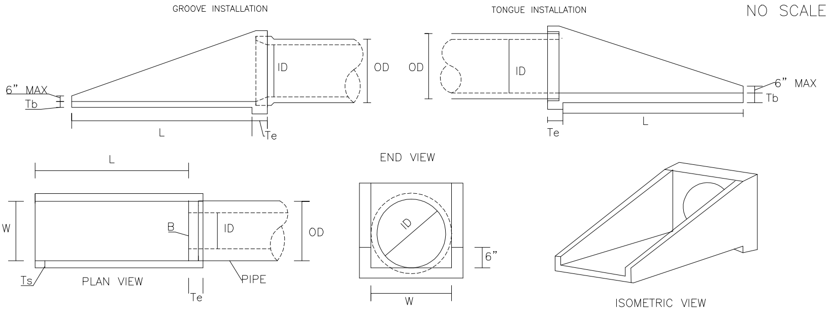
END TREATMENT DIMENSIONS
