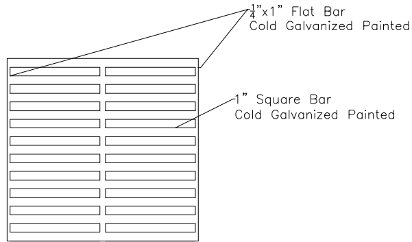
Grate Detail
