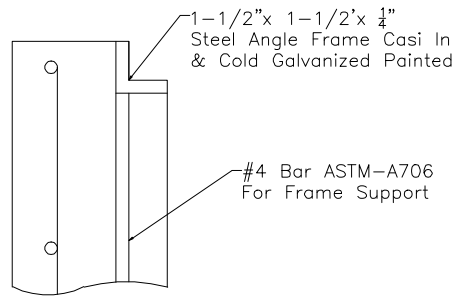
Frame Detail
