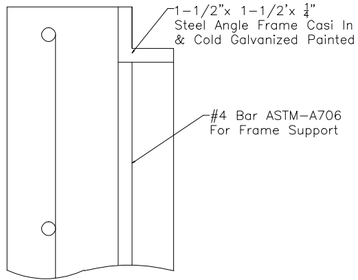
Frame Detail
