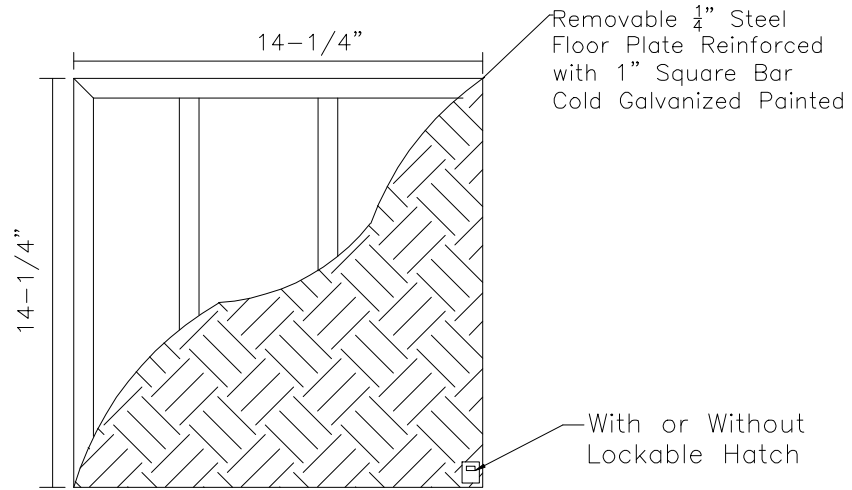
Cover Detail
